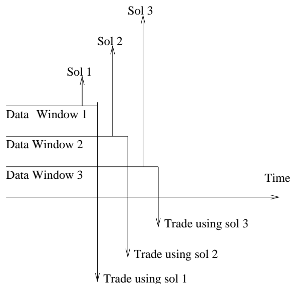
Fig. 9. An extending window approach to adaptation by updating training data.
